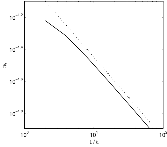
Figure 2: \eta_{h_j} versus 1/h_j in log-log scale (solid line). The dotted line with dot markers gives the reference line with slope -1/2 . The markers correspond to j = 0, 1, \dots, 5 .
