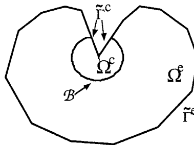
Figure 1. — Shape of the domain \Omega .
