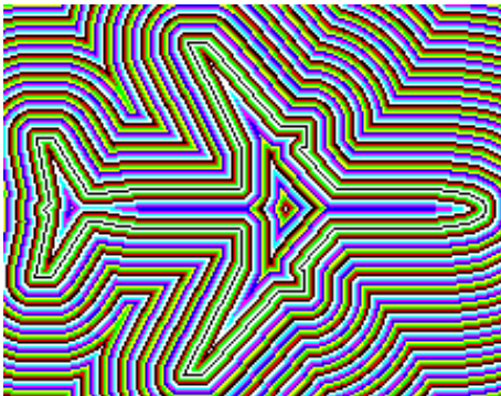
F_{(\partial^4 X)^c}^{d_E}
