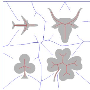
Sk_{50}(X)
