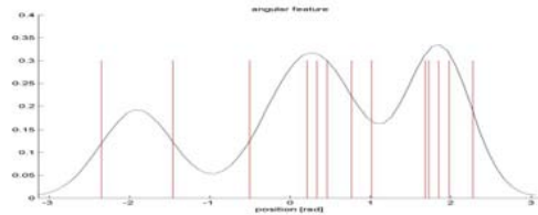
Figure 4: Evaluation of P(f=VE|loc \pi) for the original data set
