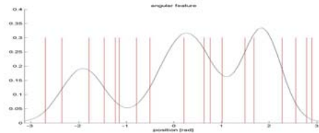
Figure 5: Evaluation of P(f=VE|loc \pi) for some other data set, resulting in a smaller value above, since the MOG is not optimal for this data.
